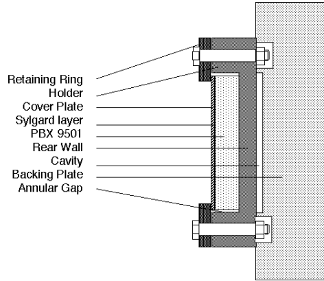
Figure 4. Basic Modified Steven target.
