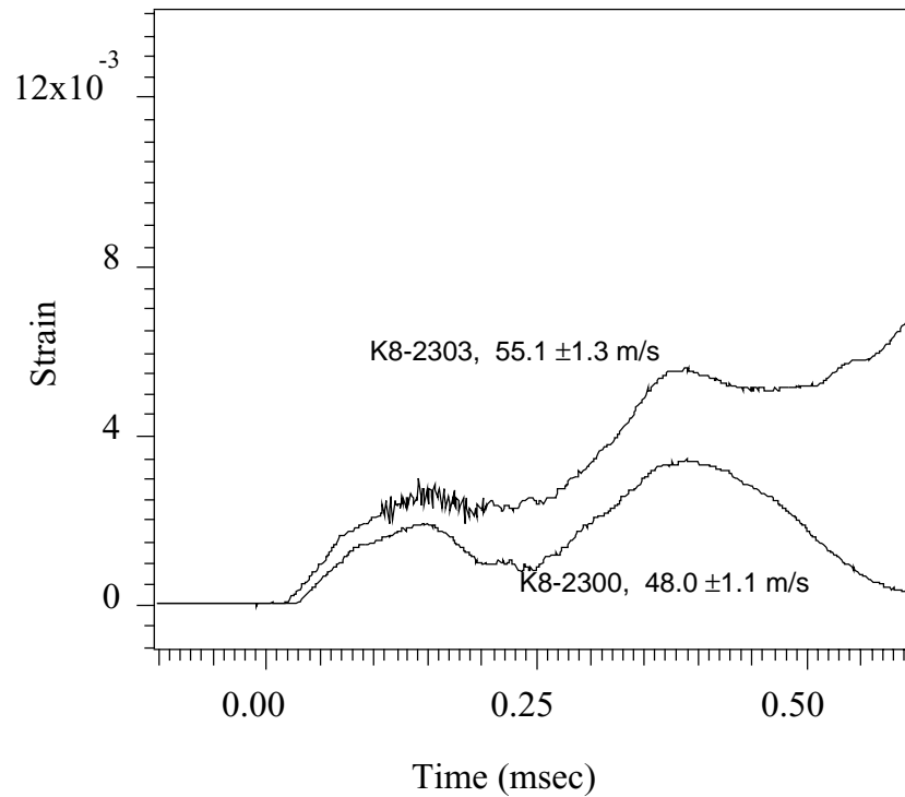
Figure 10. Examples of strain gauge records from tests K8-2300 and K8-2303. Test K8-2303 resulted in a violent reaction, and test K8-2300 was quenched.
