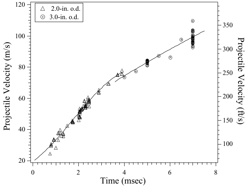
Figure 1. Powder curves.
